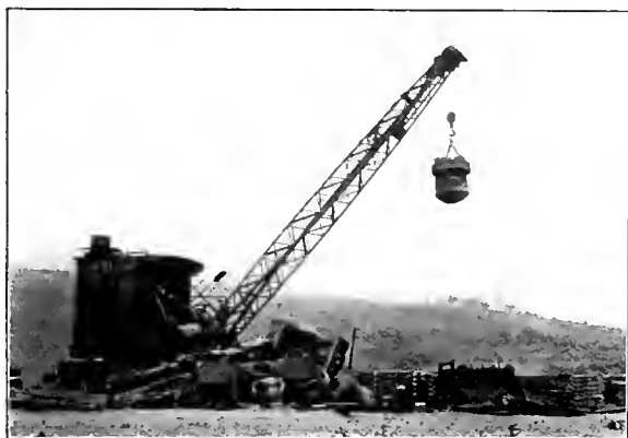
Locomotive Crane Breaking Large Scrapped Castings
